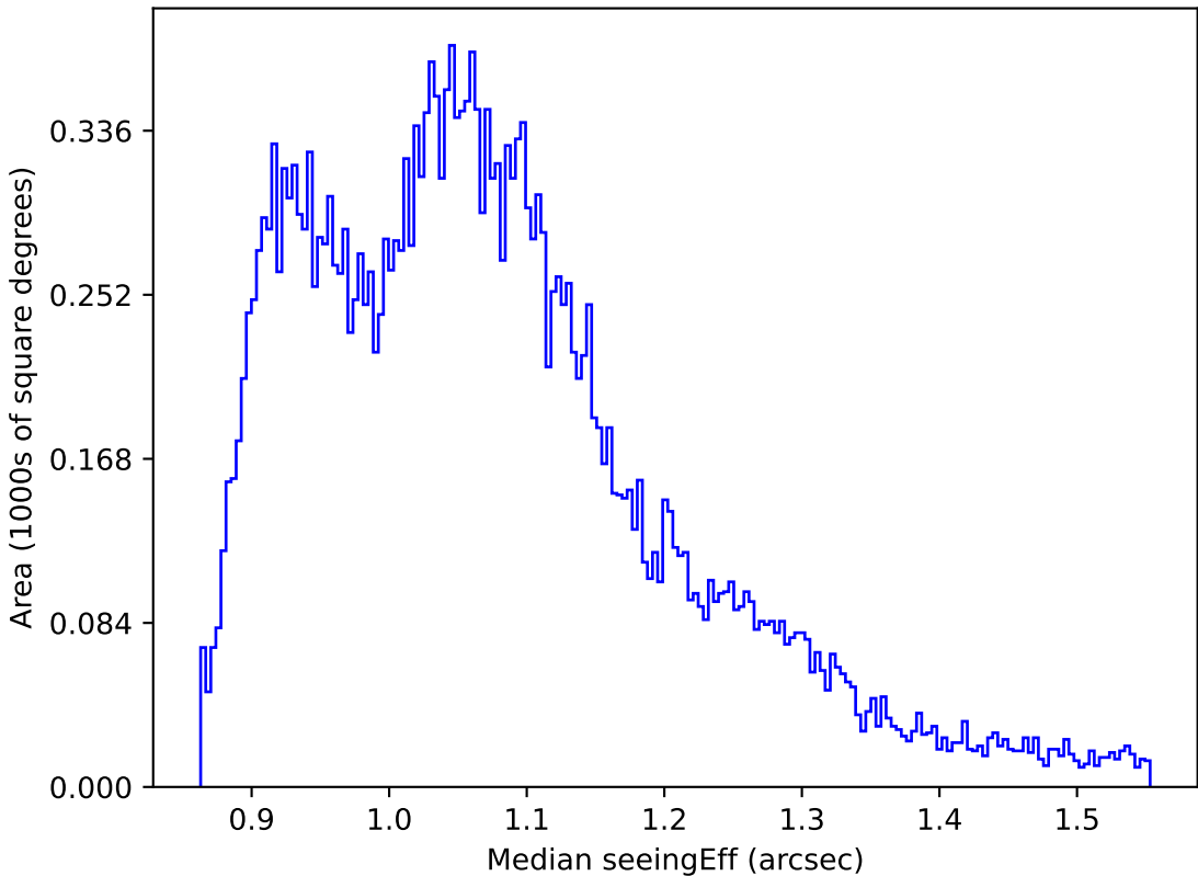
too_ignore_10_4v3.4_10yrs All sky r band: Median seeingEff
