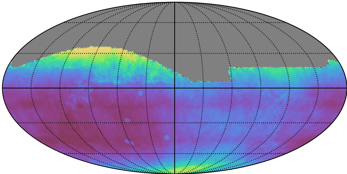
too_ignore_10_4v3.4_10yrs All sky all bands: Median seeingEff
