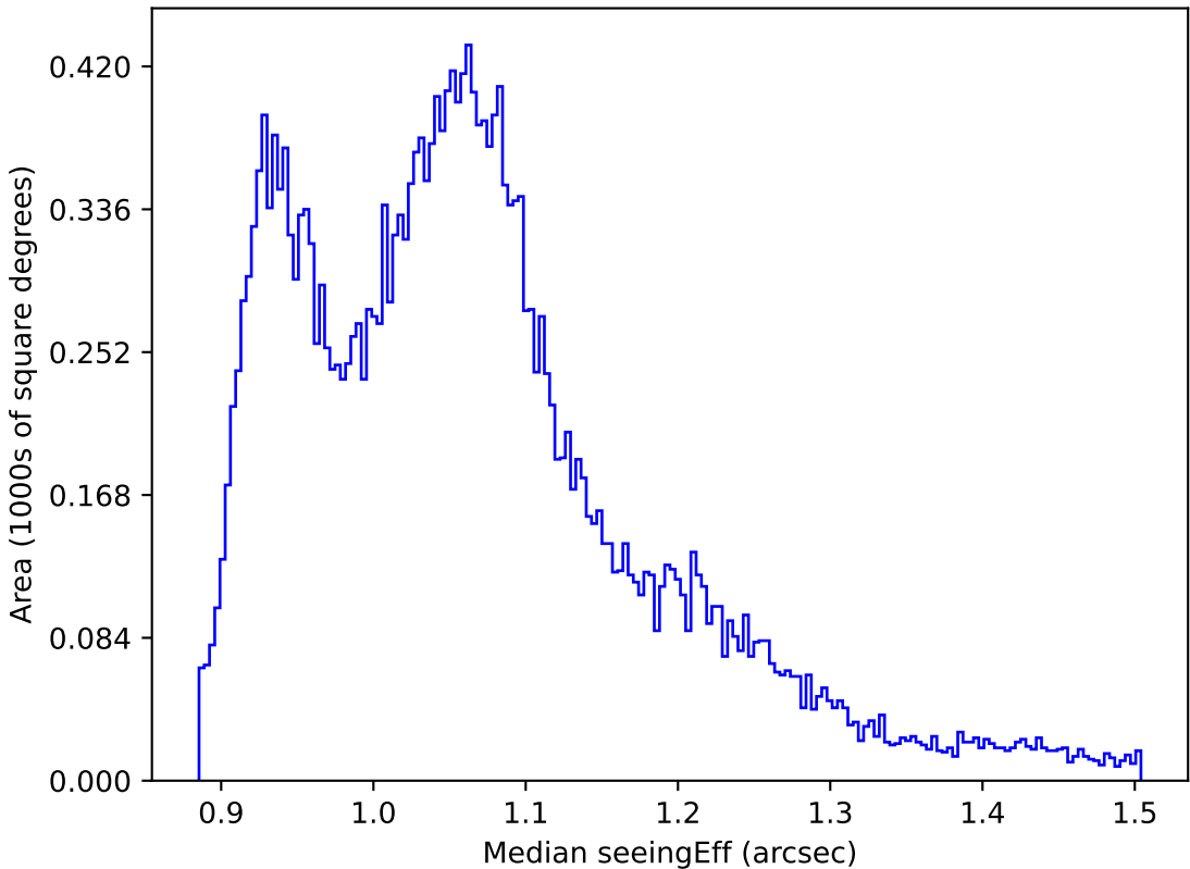
too_ignore_10_4v3.4_10yrs All sky all bands: Median seeingEff
