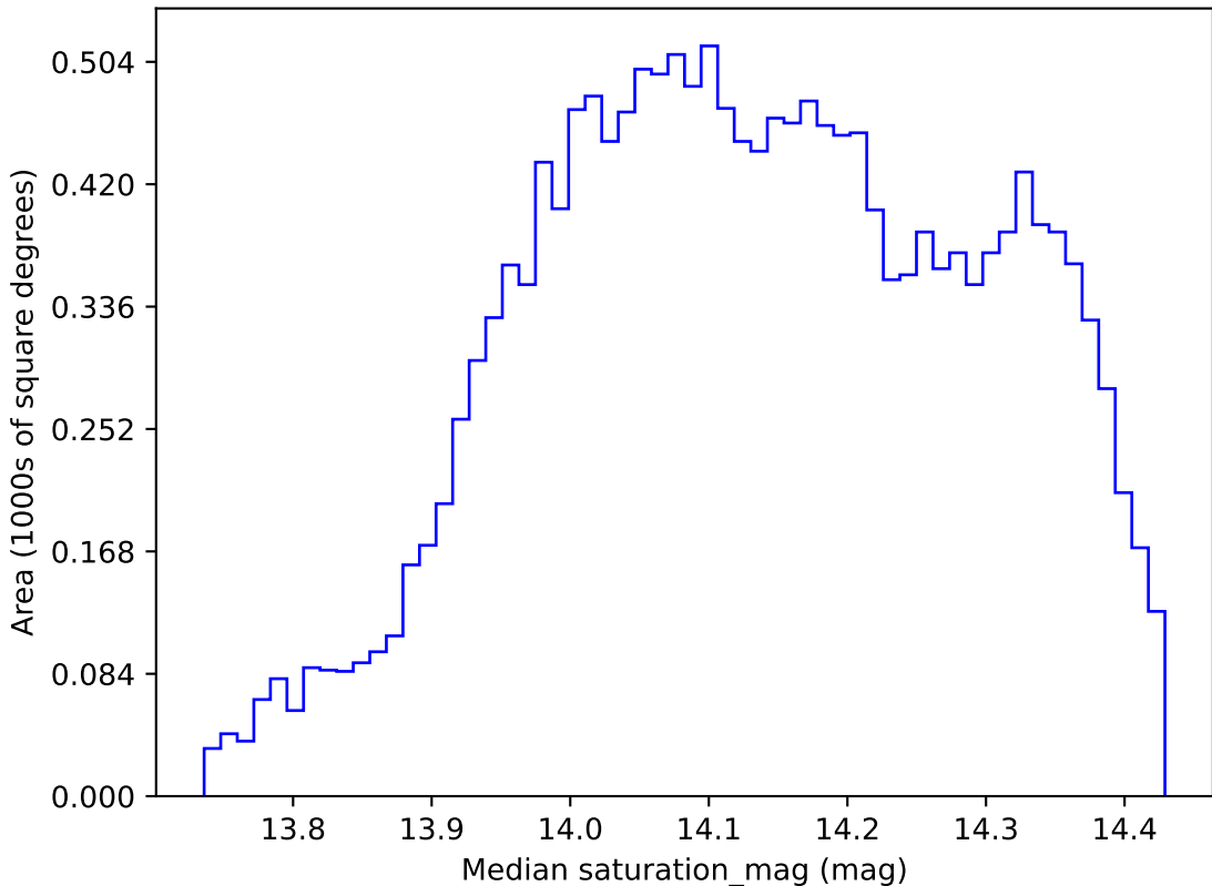
too_ignore_10_4v3.4_10yrs WFD z band: Median saturation_mag
