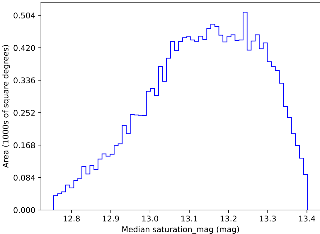
too_ignore_10_4v3.4_10yrs WFD y band: Median saturation_mag
