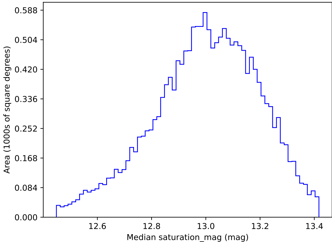
too_ignore_10_4v3.4_10yrs WFD u band: Median saturation_mag
