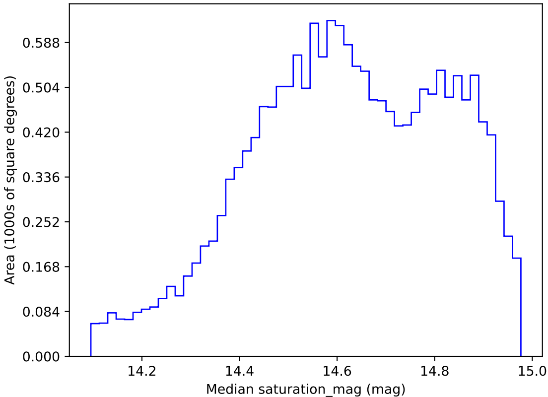
too_ignore_10_4v3.4_10yrs WFD r band: Median saturation_mag
