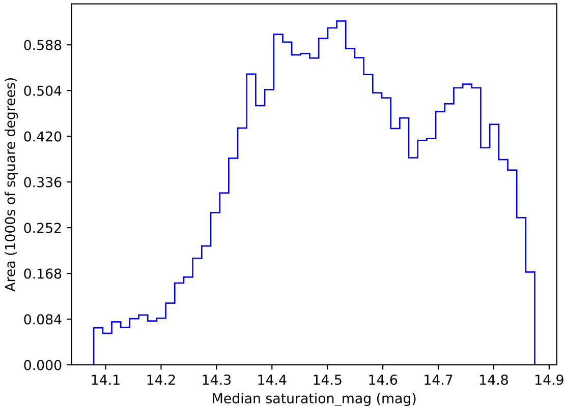
too_ignore_10_4v3.4_10yrs WFD i band: Median saturation_mag
