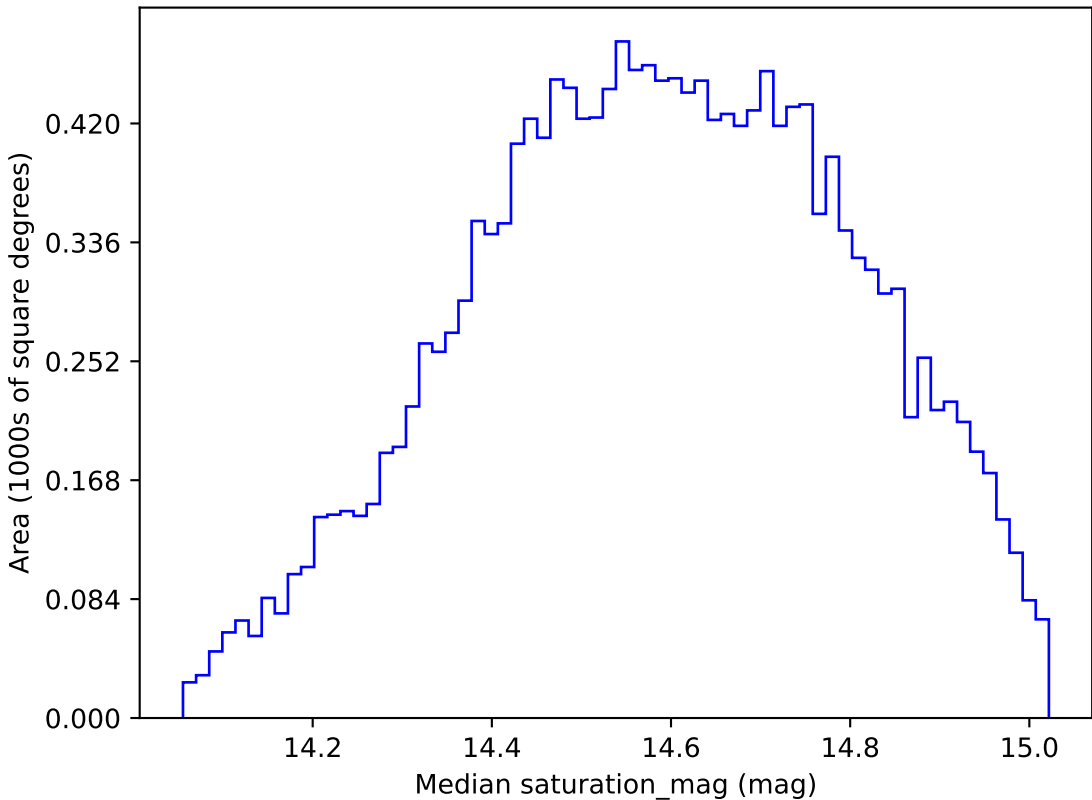
too_ignore_10_4v3.4_10yrs WFD g band: Median saturation_mag
