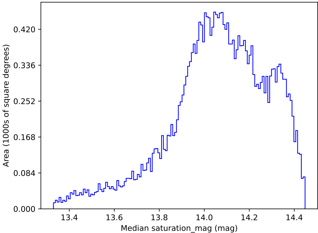
too_ignore_10_4v3.4_10yrs All sky z band: Median saturation_mag
