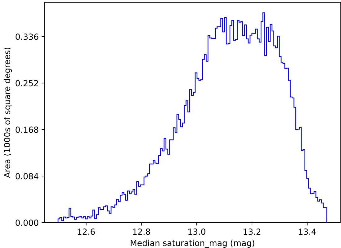
too_ignore_10_4v3.4_10yrs All sky y band: Median saturation_mag
