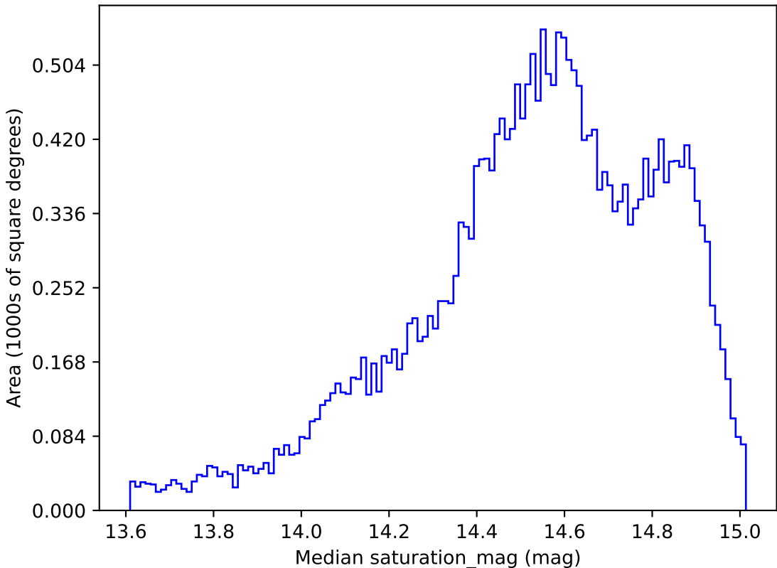
too_ignore_10_4v3.4_10yrs All sky r band: Median saturation_mag
