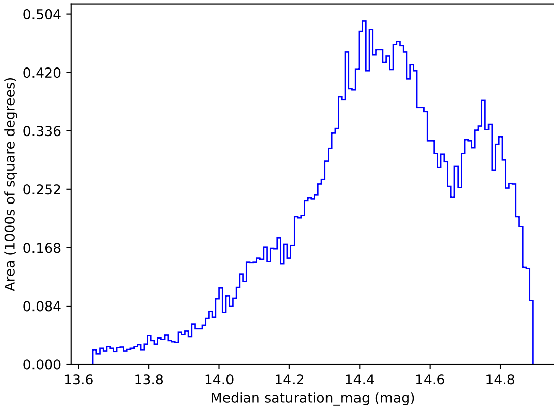
too_ignore_10_4v3.4_10yrs All sky i band: Median saturation_mag
