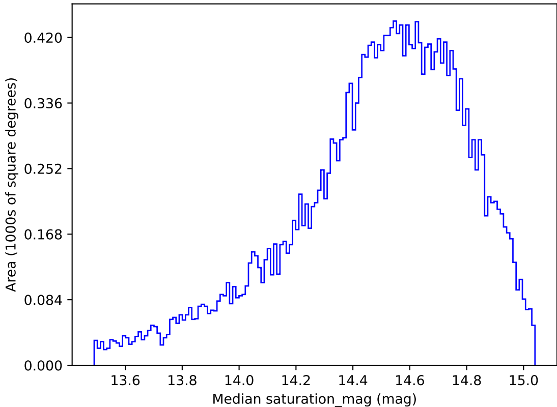
too_ignore_10_4v3.4_10yrs All sky g band: Median saturation_mag
