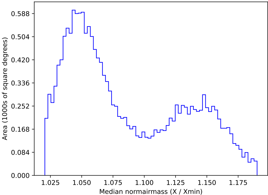
too_ignore_10_4v3.4_10yrs WFD z band: Median normairmass
