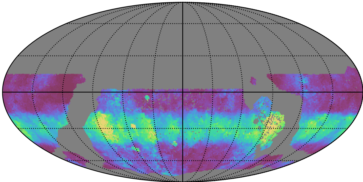
too_ignore_10_4v3.4_10yrs WFD u band: Median normairmass
