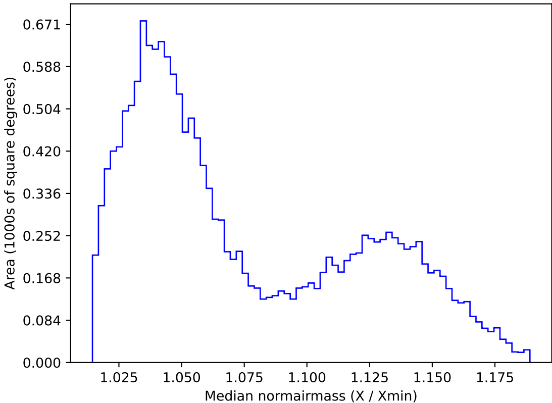
too_ignore_10_4v3.4_10yrs WFD r band: Median normairmass
