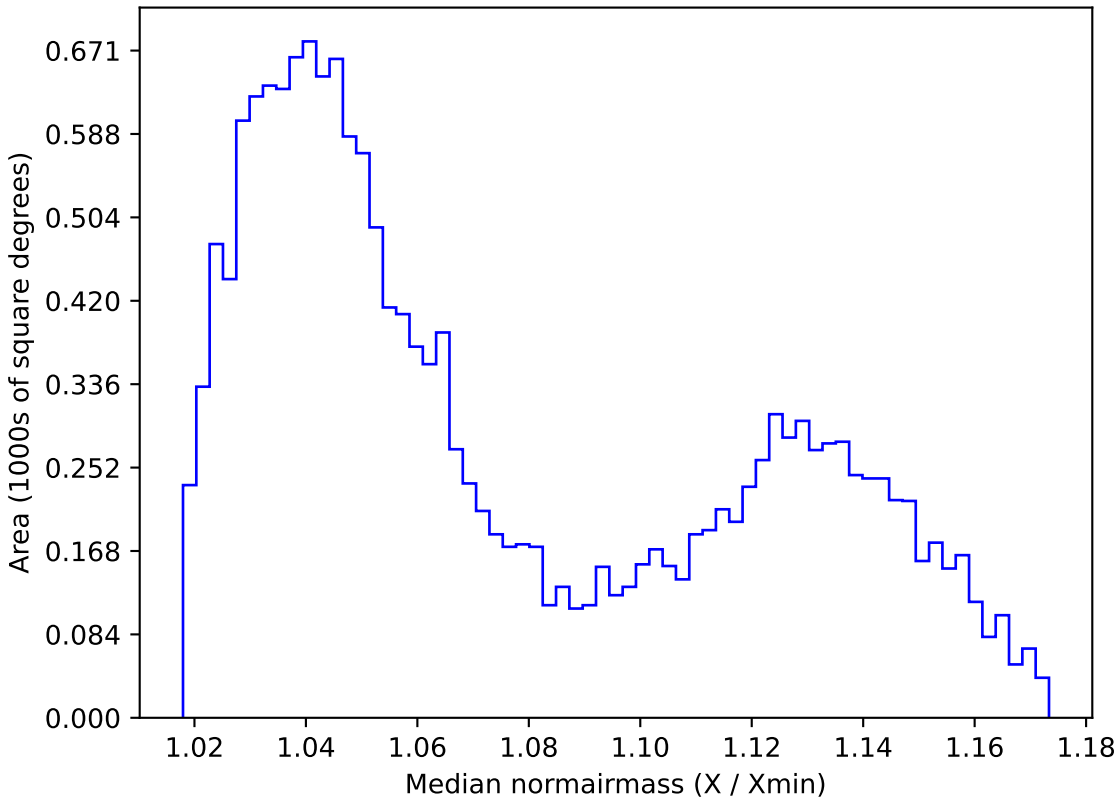
too_ignore_10_4v3.4_10yrs WFD i band: Median normairmass
