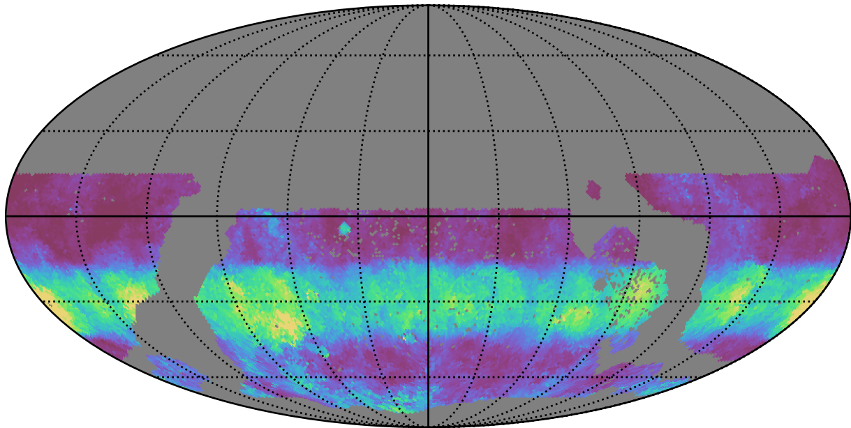
too_ignore_10_4v3.4_10yrs WFD g band: Median normairmass
