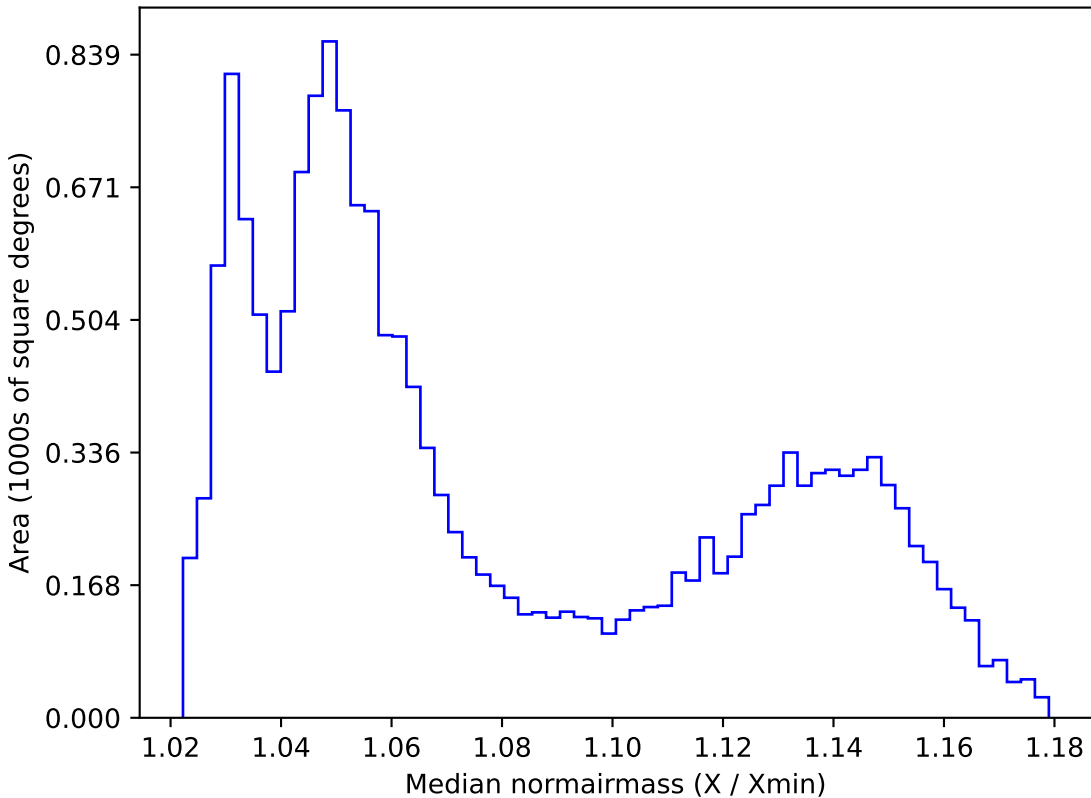
too_ignore_10_4v3.4_10yrs WFD all bands: Median normairmass
