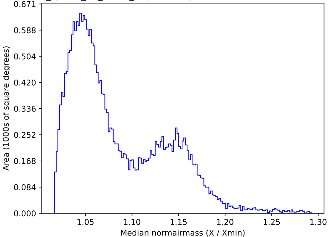
too_ignore_10_4v3.4_10yrs All sky z band: Median normairmass
