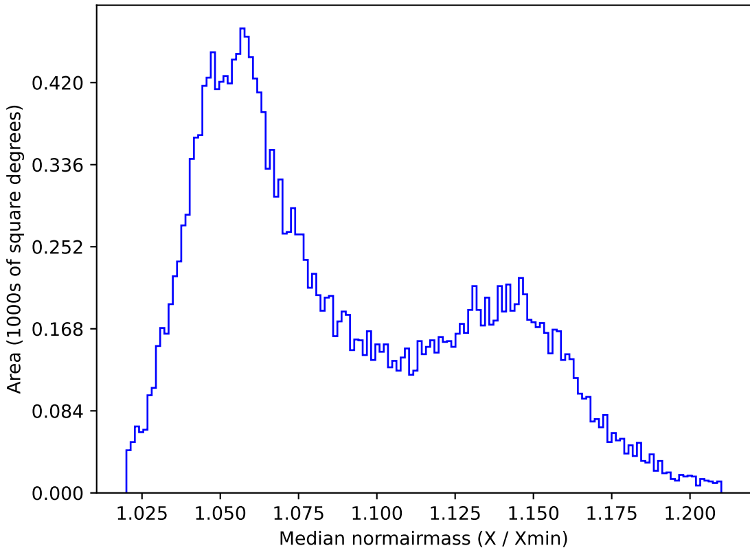
too_ignore_10_4v3.4_10yrs All sky y band: Median normairmass
