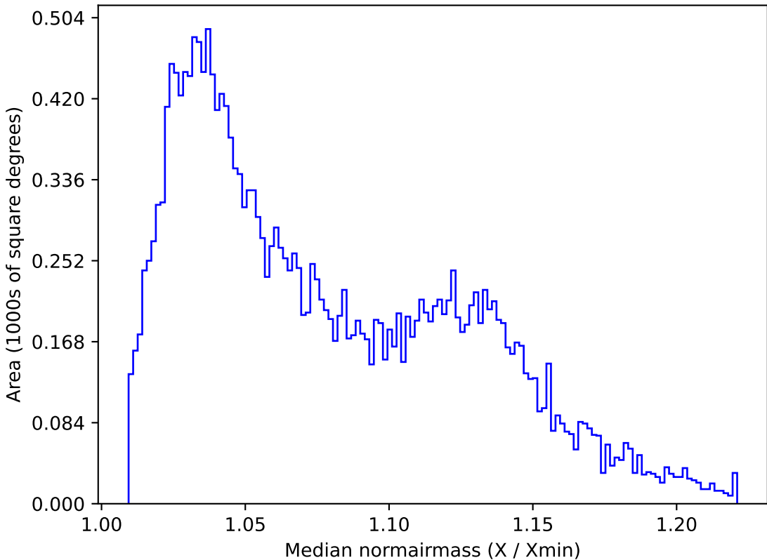
too_ignore_10_4v3.4_10yrs All sky u band: Median normairmass
