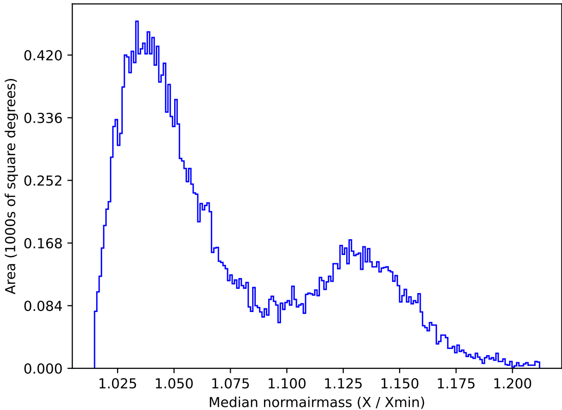
too_ignore_10_4v3.4_10yrs All sky i band: Median normairmass
