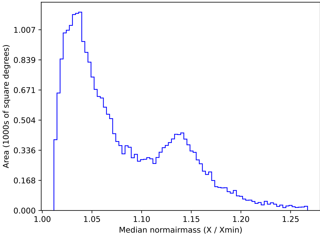
too_ignore_10_4v3.4_10yrs All sky g band: Median normairmass
