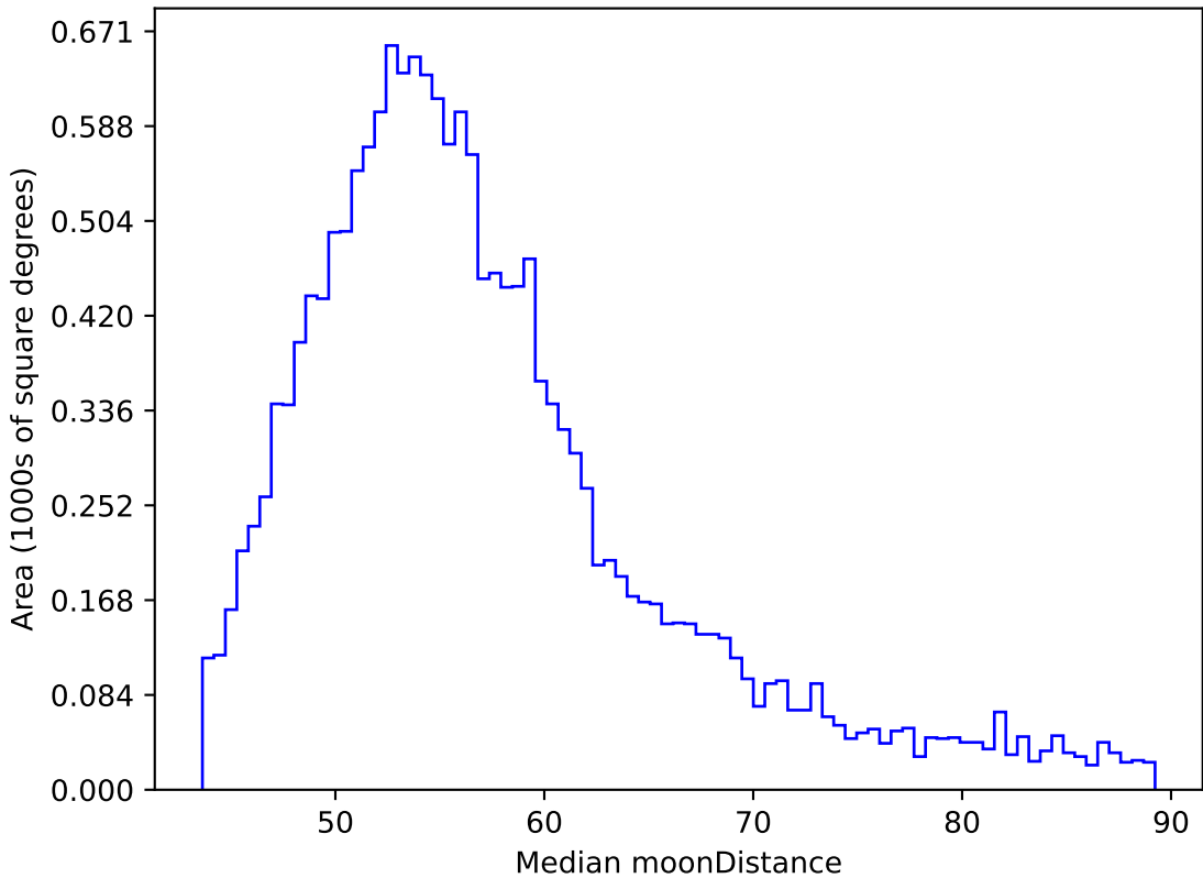
too_ignore_10_4v3.4_10yrs WFD y band: Median moonDistance
