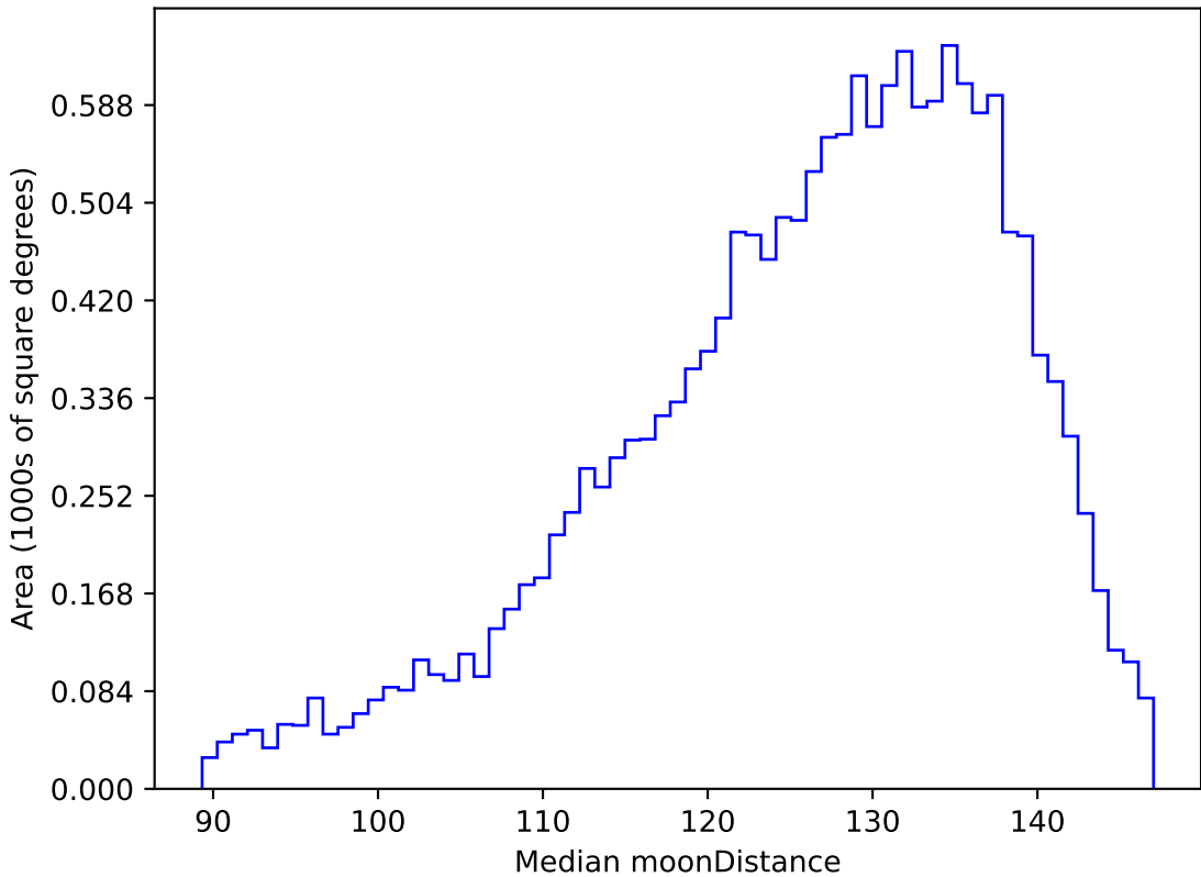
too_ignore_10_4v3.4_10yrs WFD u band: Median moonDistance
