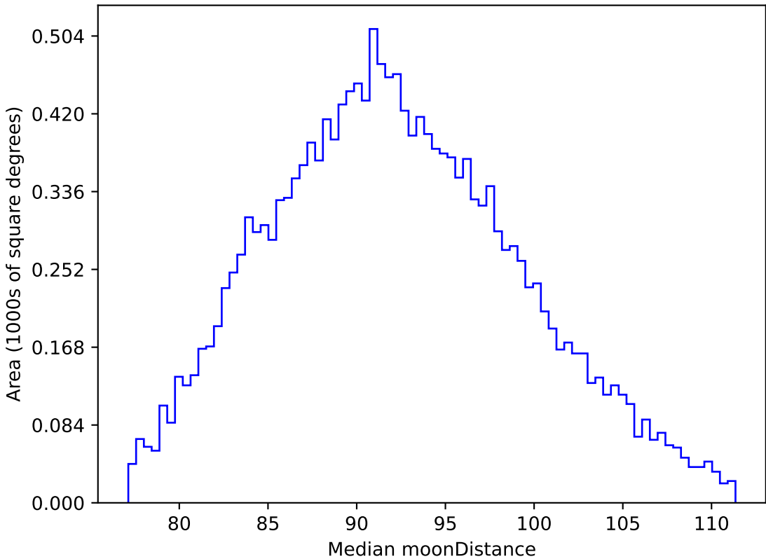
too_ignore_10_4v3.4_10yrs WFD i band: Median moonDistance
