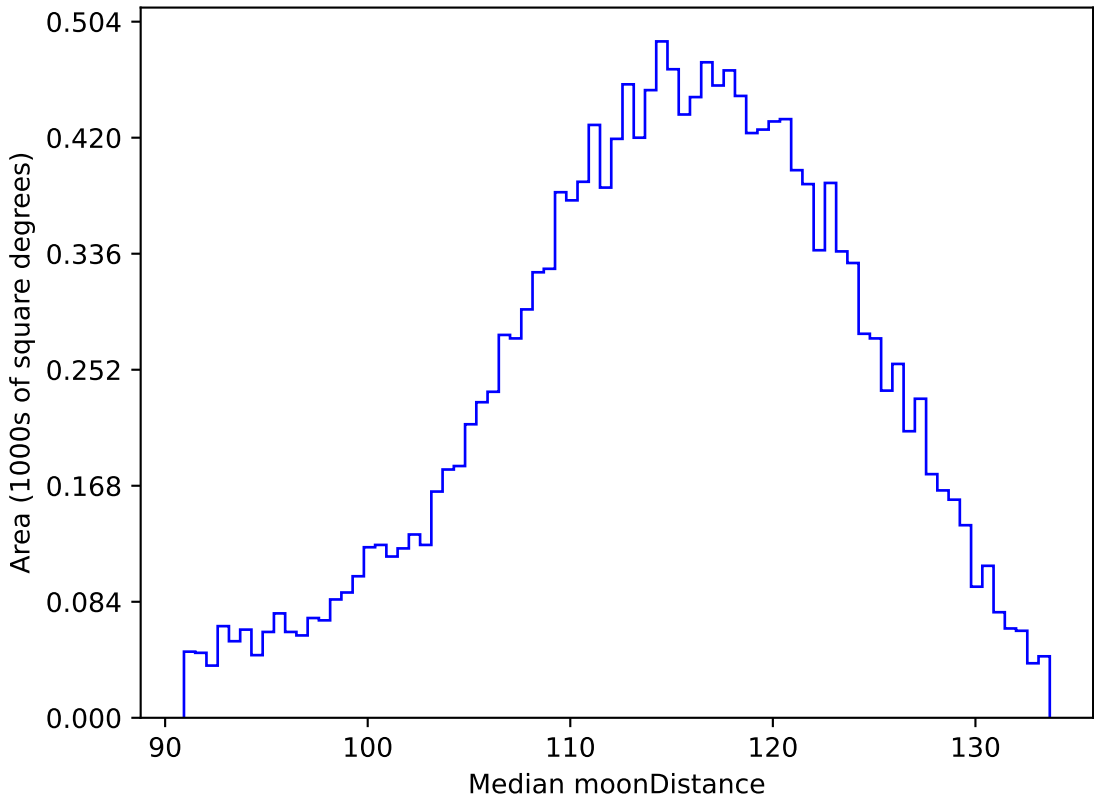
too_ignore_10_4v3.4_10yrs WFD g band: Median moonDistance
