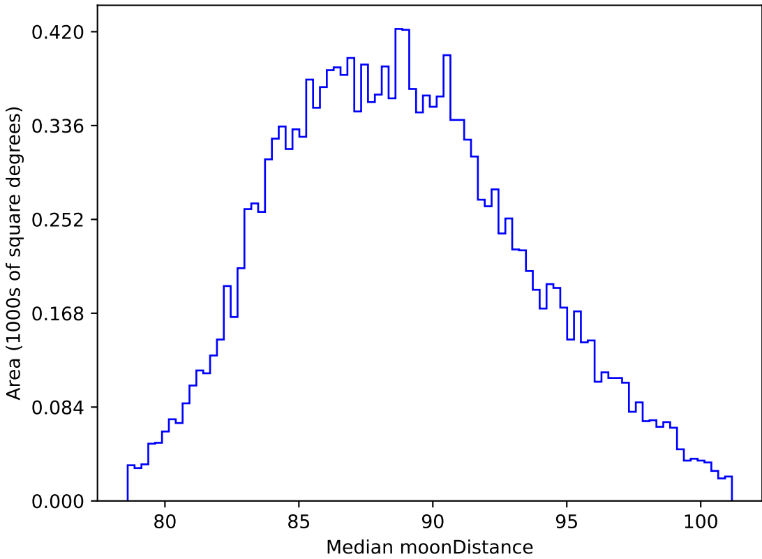
too_ignore_10_4v3.4_10yrs WFD all bands: Median moonDistance
