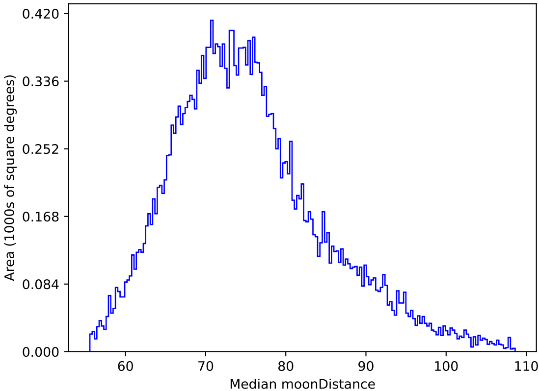
too_ignore_10_4v3.4_10yrs All sky z band: Median moonDistance
