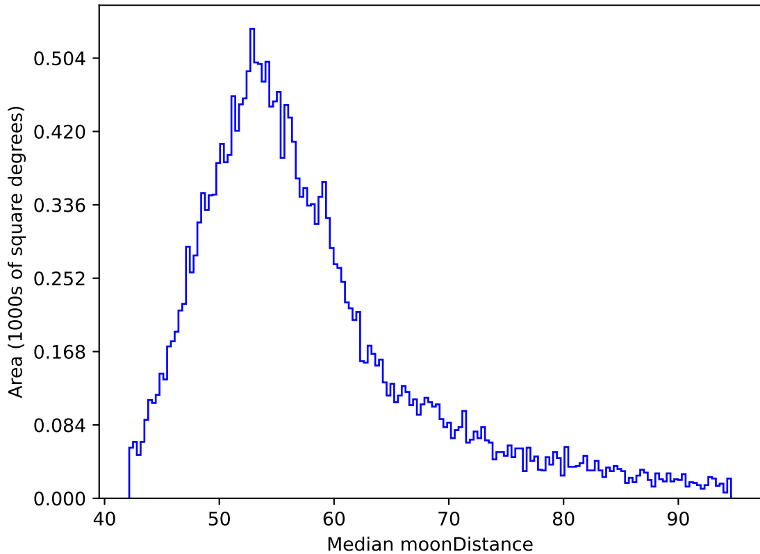
too_ignore_10_4v3.4_10yrs All sky y band: Median moonDistance
