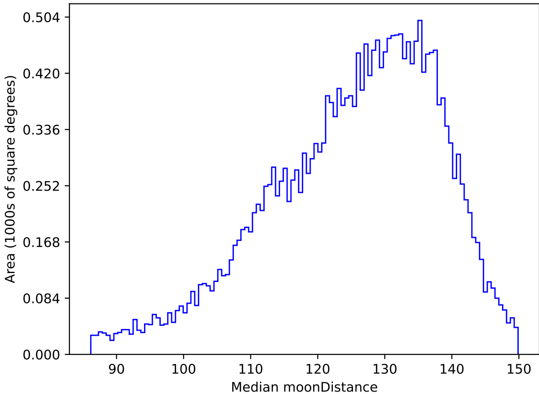
too_ignore_10_4v3.4_10yrs All sky u band: Median moonDistance
