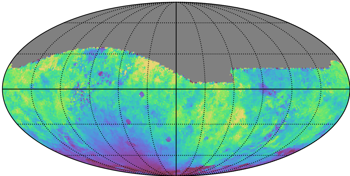
too_ignore_10_4v3.4_10yrs All sky r band: Median moonDistance
