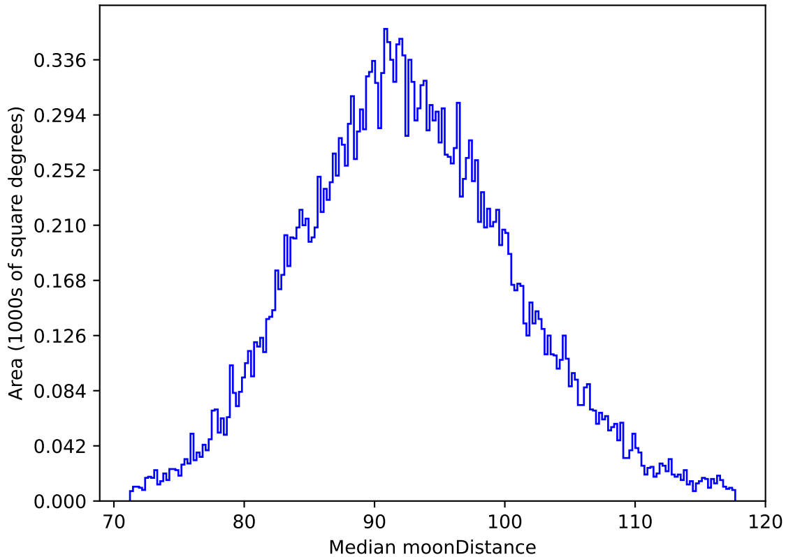
too_ignore_10_4v3.4_10yrs All sky i band: Median moonDistance
