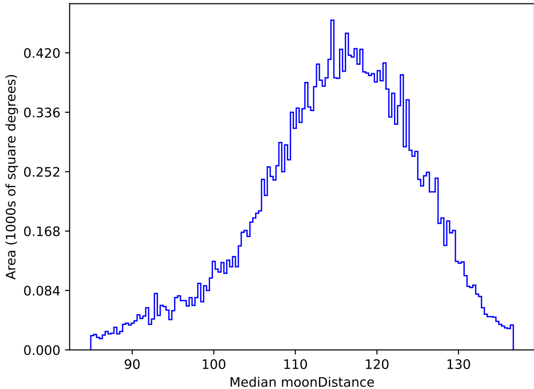
too_ignore_10_4v3.4_10yrs All sky g band: Median moonDistance
