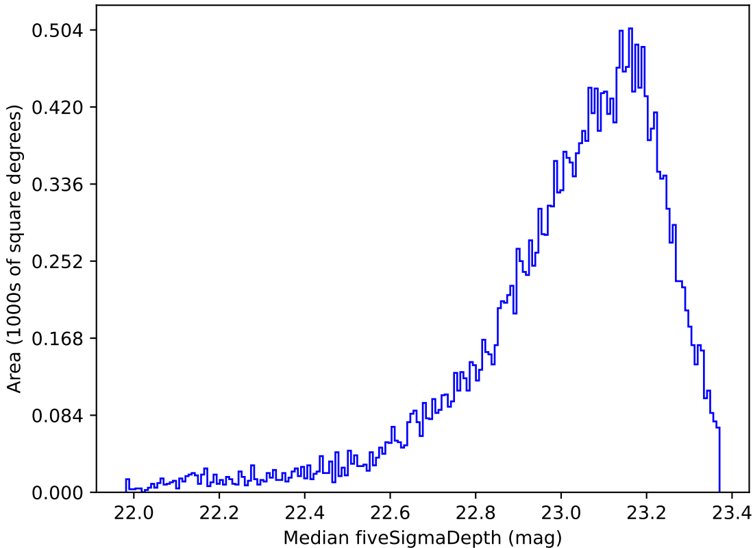
too_ignore_10_4v3.4_10yrs Yr 1 z band: Median fiveSigmaDepth
