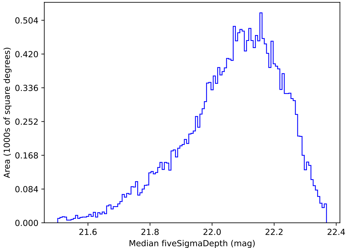
too_ignore_10_4v3.4_10yrs Yr 1 y band: Median fiveSigmaDepth
