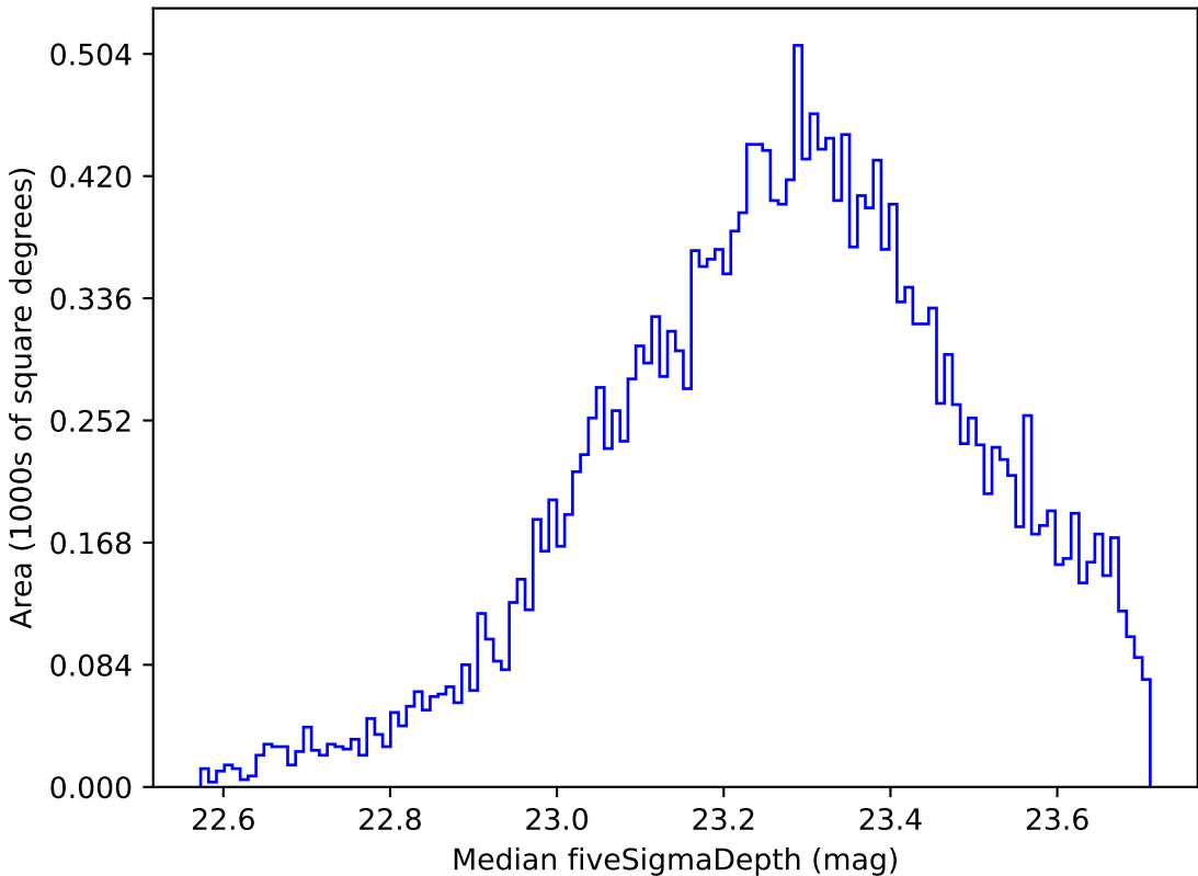
too_ignore_10_4v3.4_10yrs Yr 1 u band: Median fiveSigmaDepth
