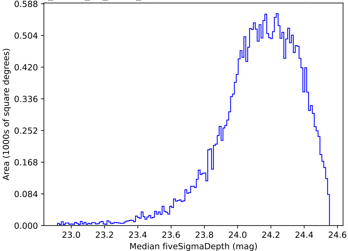
too_ignore_10_4v3.4_10yrs Yr 1 r band: Median fiveSigmaDepth
