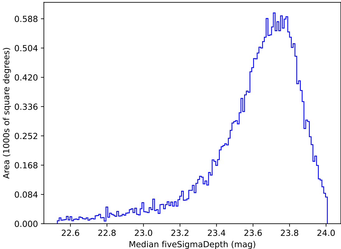
too_ignore_10_4v3.4_10yrs Yr 1 i band: Median fiveSigmaDepth
