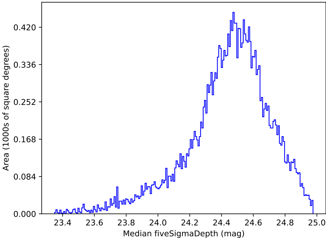
too_ignore_10_4v3.4_10yrs Yr 1 g band: Median fiveSigmaDepth
