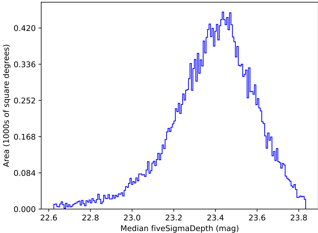
too_ignore_10_4v3.4_10yrs Yr 1 all bands: Median fiveSigmaDepth
