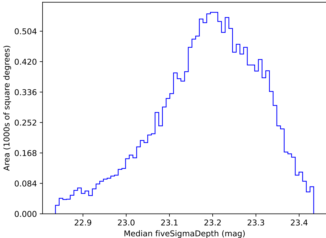
too_ignore_10_4v3.4_10yrs WFD u band: Median fiveSigmaDepth
