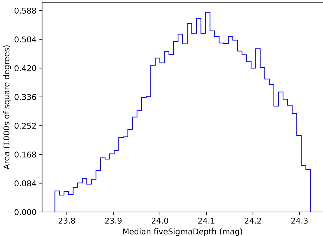
too_ignore_10_4v3.4_10yrs WFD r band: Median fiveSigmaDepth
