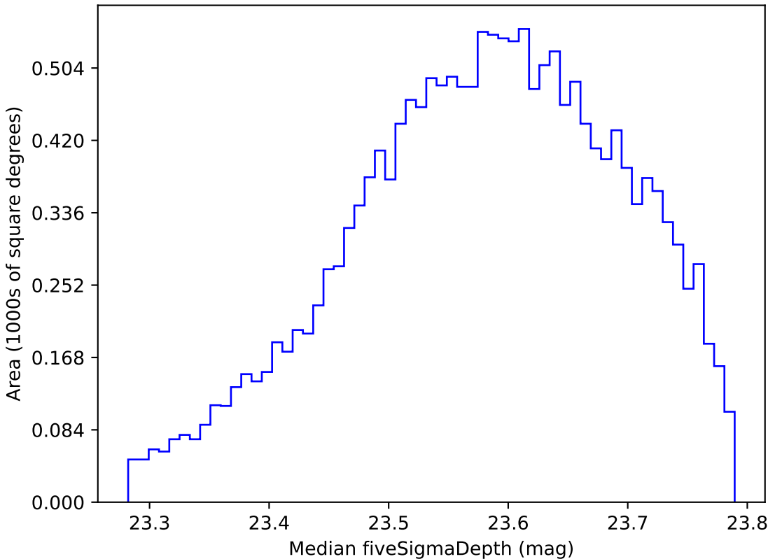
too_ignore_10_4v3.4_10yrs WFD i band: Median fiveSigmaDepth
