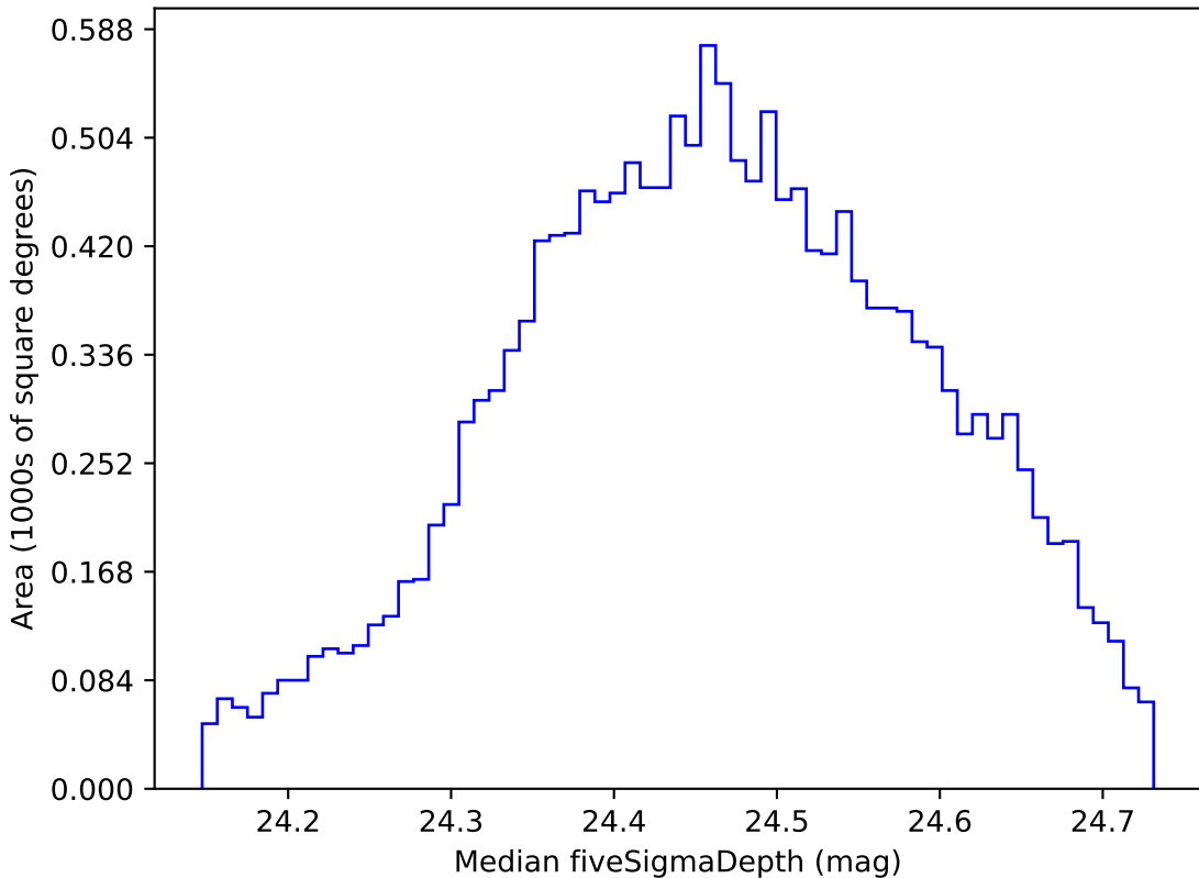
too_ignore_10_4v3.4_10yrs WFD g band: Median fiveSigmaDepth
