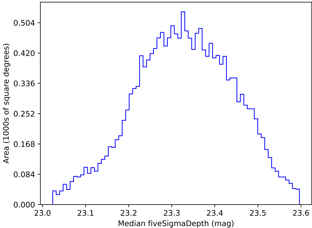
too_ignore_10_4v3.4_10yrs WFD all bands: Median fiveSigmaDepth
