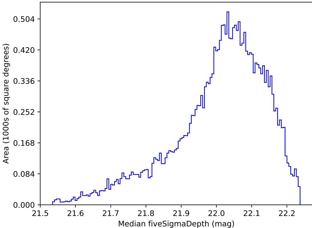
too_ignore_10_4v3.4_10yrs All sky y band: Median fiveSigmaDepth
