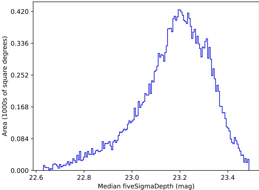
too_ignore_10_4v3.4_10yrs All sky u band: Median fiveSigmaDepth
